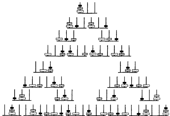
Figure 2 Problem Space for the Three-Disk Tower of Hanoi Problem
